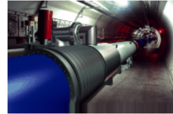
LHC (2007)
