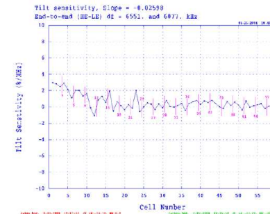
Tilt Sensitivity
