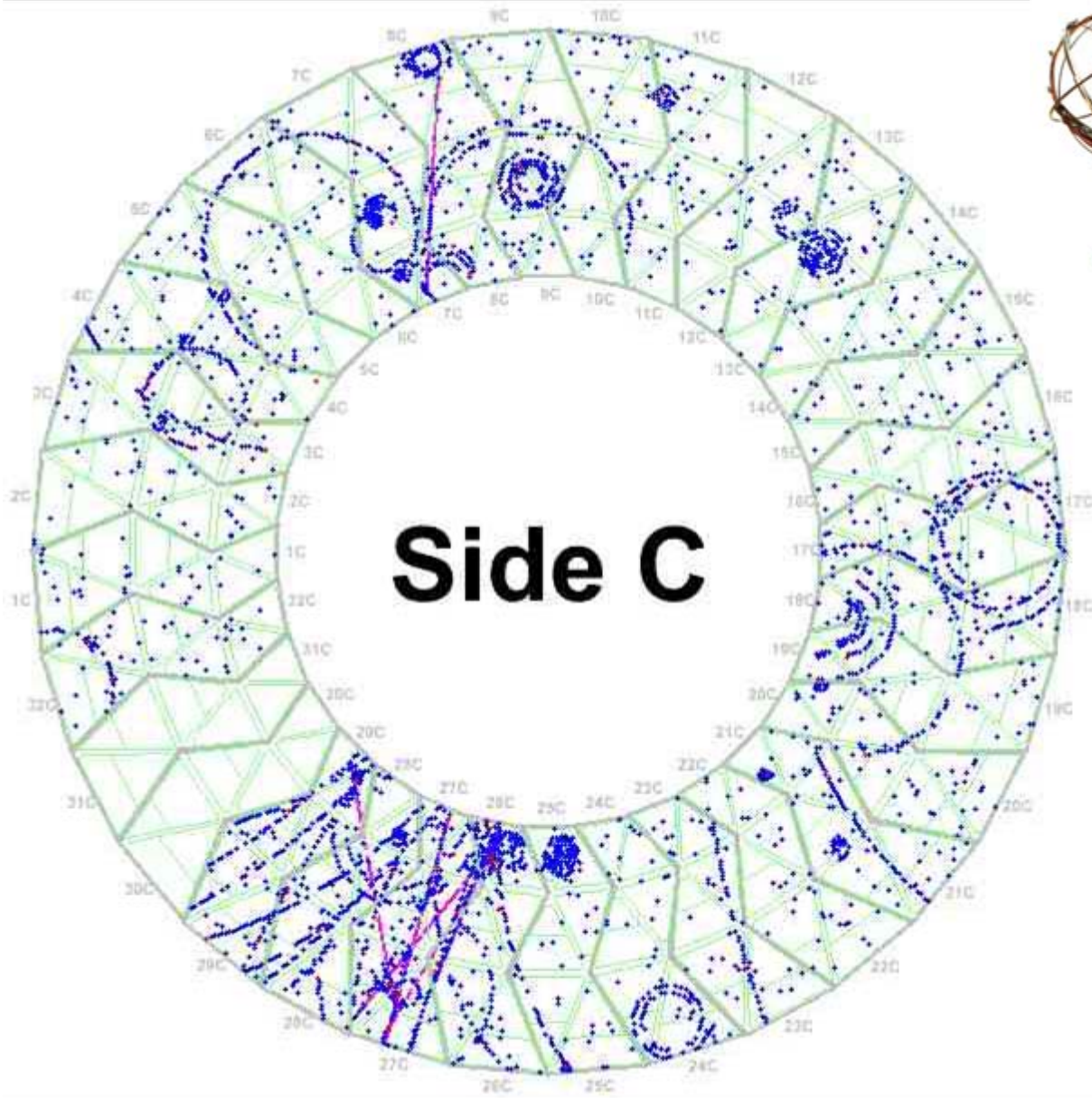
Run 50905 Event 1576, y vs x
