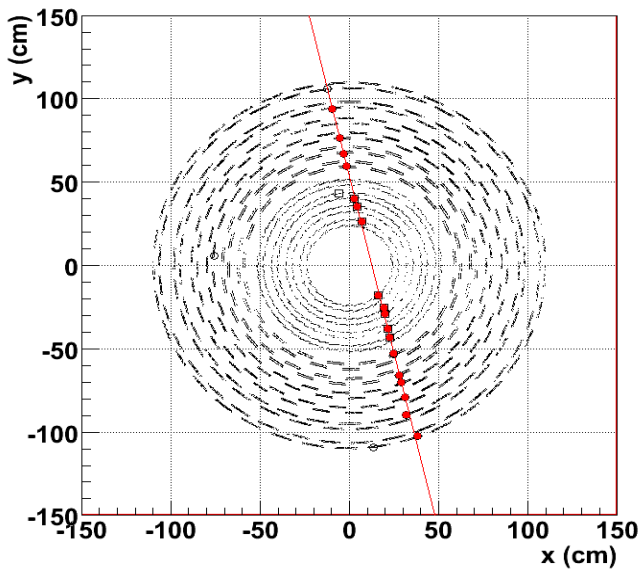
Run 50905 Event 1576, y vs x
