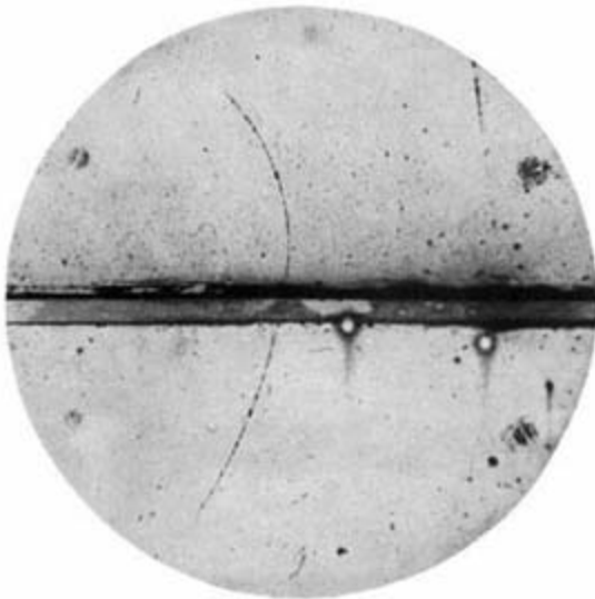
FIG. 1. A 63 million volt positron ( H_0=2.1 \times 10^6 gauss-cm) passing through a 6 mm lead plate and emerging as a 23 million volt positron ( H_0=1.3 \times 10^6 gauss-cm). The length of this latter path is at least ten times greater than the possible length of a proton path of this curvature.
